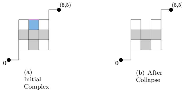
Figure 11: The LPDC for the window that changes dipath space. The LPDC of the edge [(2, 4), (3, 4)] changes the dipath space between \mathbf{0} to (5, 5) from having six connected components to five connected components.
