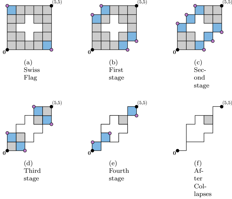
Figure 4: Collapsing the Swiss Flag. A sequence of vertex collapses is presented from the top left to bottom right. At each stage of the sequence, the faces and vertices shaded in blue and purple represent the vertex collapsing pairs with the blue Euclidean cube being \sigma and the purple vertex being \tau . The result of the sequence of LPDCs is shown in (f) is a one-dimensional directed Euclidean cubical complex and one two-cube. Observe that this directed Euclidean cubical complex clearly illustrates the two dihomotopy classes of \vec{P}_0^{(5,5)}(K) .
