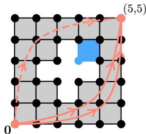
Figure 1: The Swiss Flag and Three Directed Paths. The gray and blue squares are the two-cubes of a Euclidean cubical complex. The bi-monotone increasing paths are directed paths starting at (0, 0) and ending at (5, 5) . This complex has a cross-shaped hole in the middle. As a consequence, the solid directed paths are directed homotopic while the dashed directed path is not directed homotopic to either of the other directed paths. Each point highlighted in blue is unreachable , meaning that we cannot reach any point highlighted in blue without breaking bi-monotonicity in a path starting at (0, 0) . This complex models the dining philosophers problem, a well-known example in concurrency, where two processes require two shared resources with limited capacity [4, 12]. The two distinct paths (solid and dashed) represent which process uses both shared resources first.
